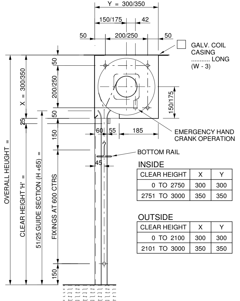
TYPICAL SECTION
