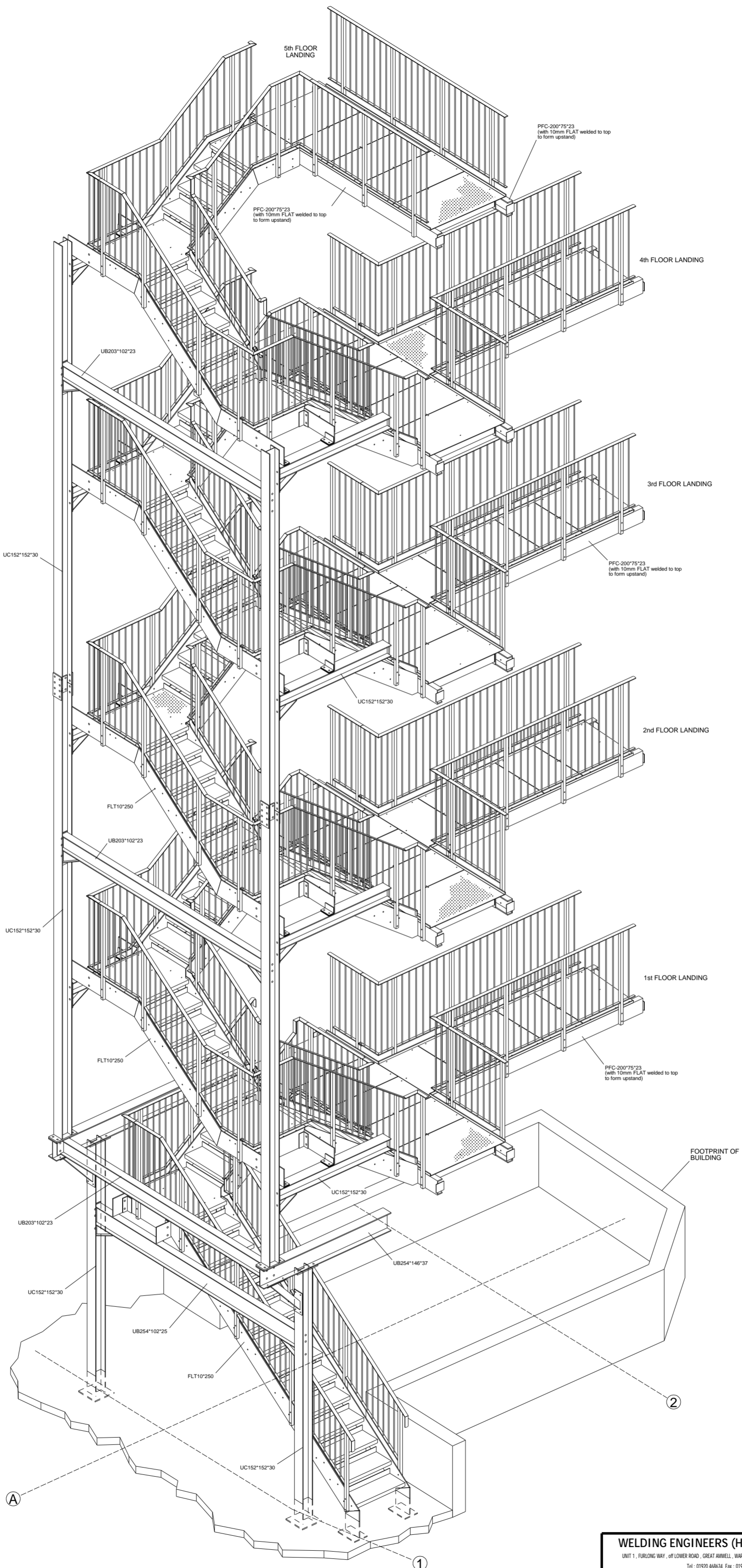
FULL ISOMETRIC VIEW
